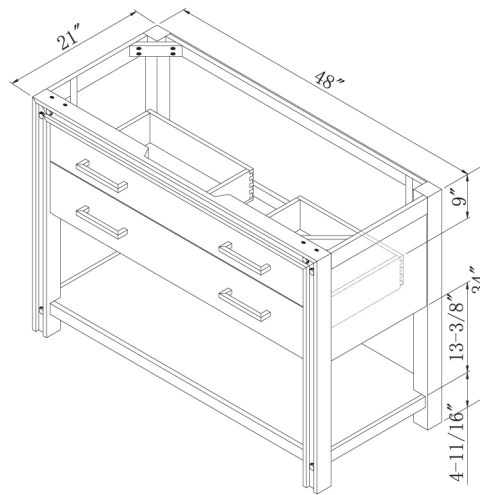
UM4821D Vanity 1 x Drawer
