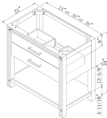
UM2421D/UM3021D/UM3621D Vanity 1 x Drawer
