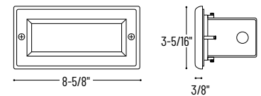
NSW-842/32 Lensed
