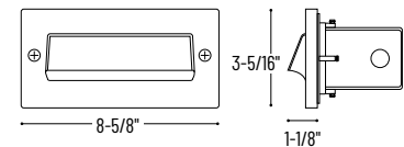
NSW-843/32 Shroud
