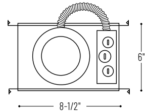
4-3/8" Ceiling Cut-out
