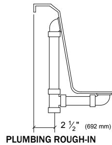
PLUMBING ROUGH-IN
