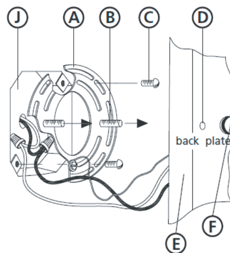
Drawing 2 – Installation
