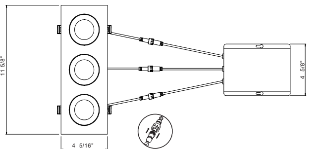
PRODUCT DIMENSIONS
