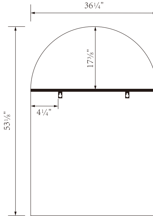
Back View
