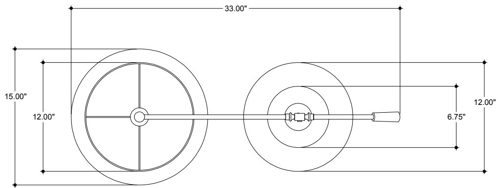
TOP VIEW
