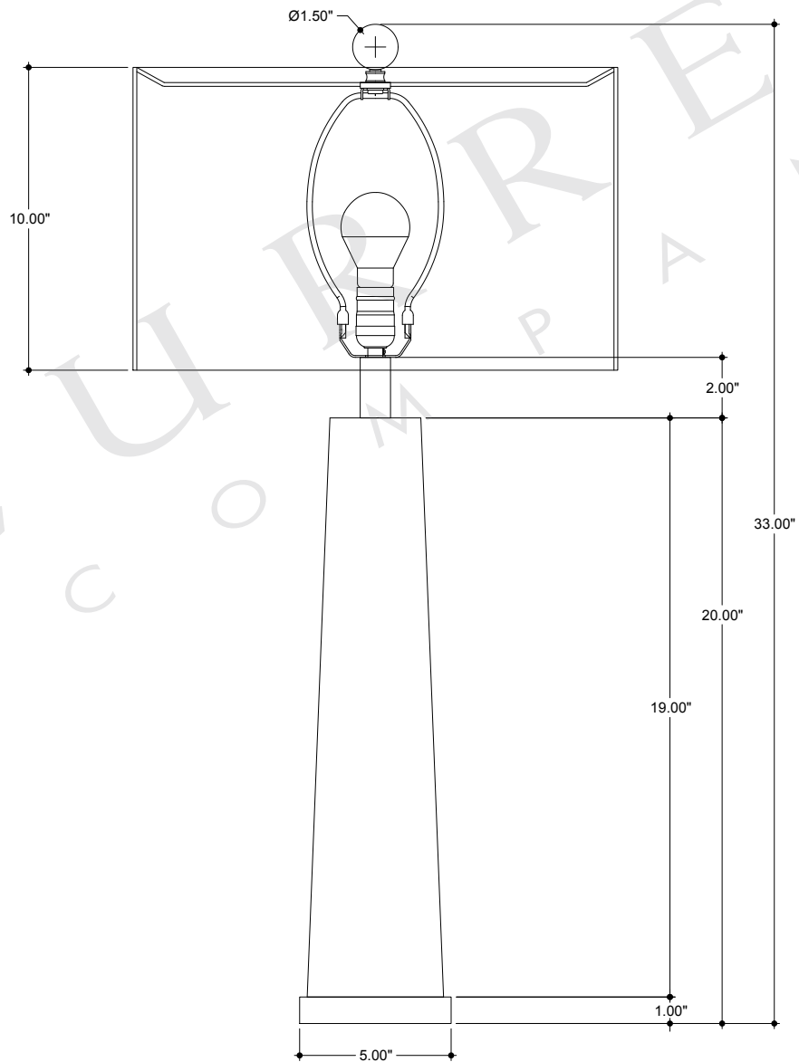
FRONT VIEW
