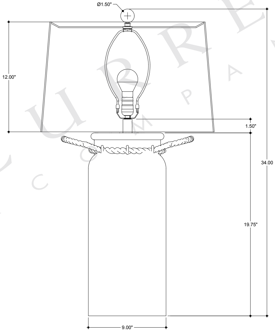
FRONT VIEW
